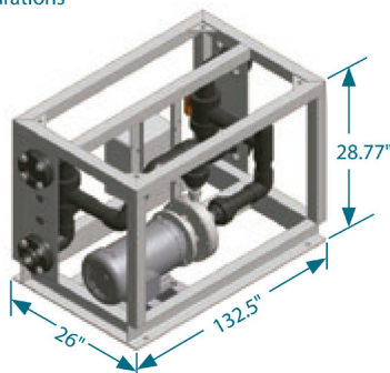
BOOSTER PUMP SKID
