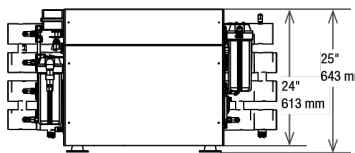
Compact frontal
