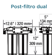
Post-filtro dual
