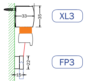
2 BAR FOOTPLATE FACE FIXED BLIND Types: A0-DB, A0-DBE,
