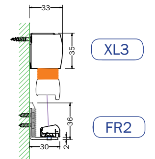
3 Bar FACE FIXED BLIND Types: A0-DB, A0-DBE, AB, DB, DBE, PB
