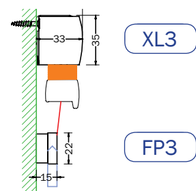
2 BAR FOOTPLATE FACE FIXED BLIND Types: A0-DB, A0-DBE,
