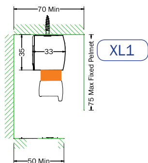
2 BAR RECESS FIXED BLIND Type: A0
