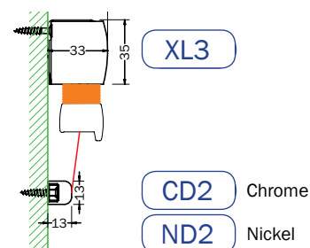
2 BAR CHROME DOME FACE FIXED BLIND Types: A0-DB, A0-DBE,
