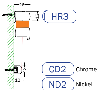
2 BAR DOME FACE FIXED BLIND Types: AO-DB, AO-DBE, AB, DB, DBE, PB
