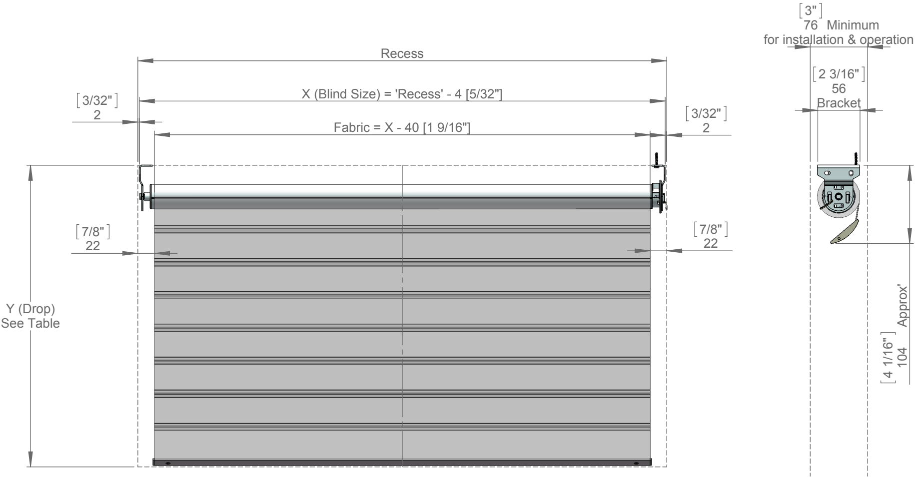
VIEW FROM INBOARD
