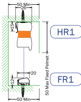
3 BAR RECESS FIXED BLIND Types: AO-DB, AO-DBE, AB, DB, DBE, PB
