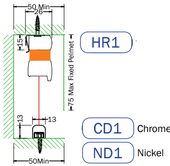
2 BAR DOME RECESS FIXED BLIND Types: AO-DB, AO-DBE, AB, DB, DBE, PB
