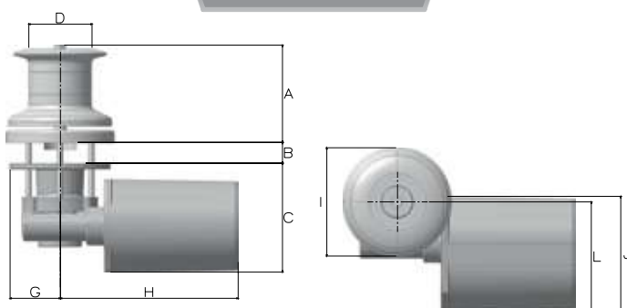
Dimensions (mm)
